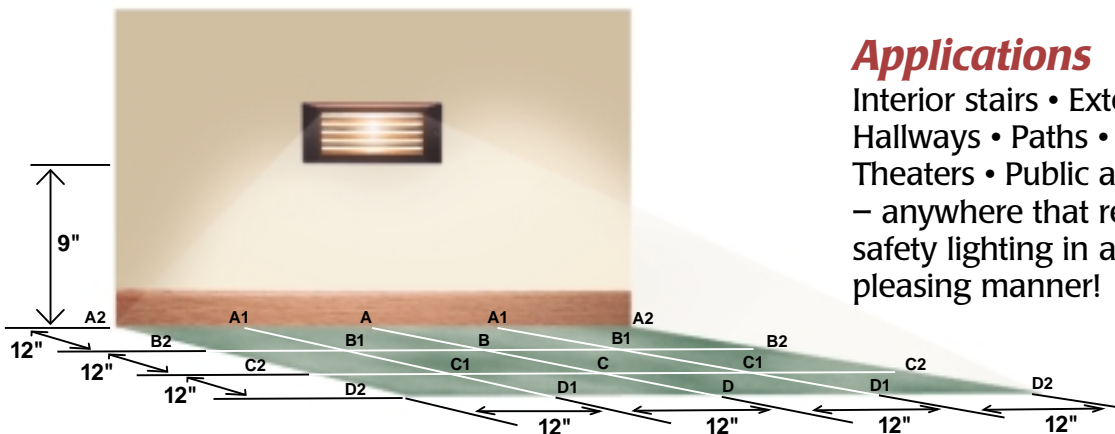
Xenon Brick Light
