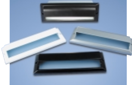
Scoop Cover: White, Black, Bronze, Aluminum Cover: 9"L x 3"W x 1.5"D Can: 7.7"L x 2.4"W x 3.2"D
