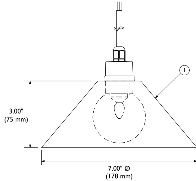
Part#: EX-CS2-B shown w/G-19 Globe
