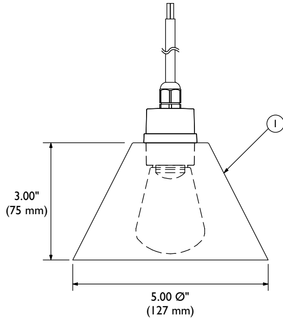
Part#: EX-CS1-B shown w/S-14 Globe
