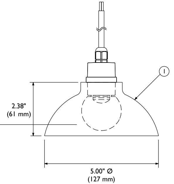
Part#: EX-CS3-B shown w/G-14Globe
