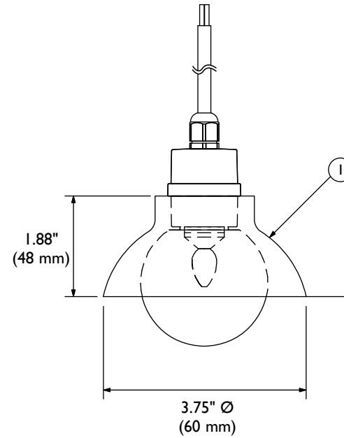
Part#: EX-CS3-B shown w/G-19 Globe
