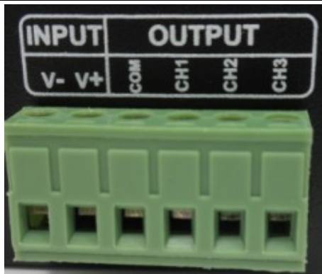
Adopt 6 pin screw as power and load interface
